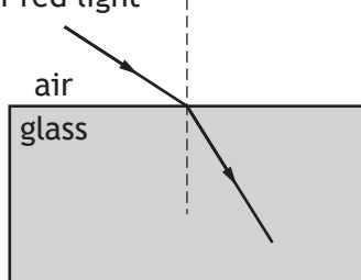
C ray of red light
