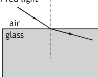
A ray of red light
