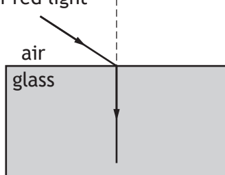
D ray of red light
