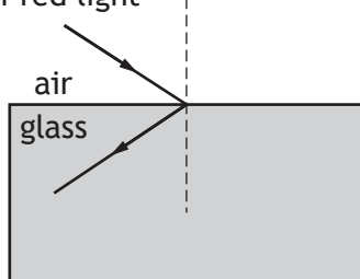
E ray of red light
