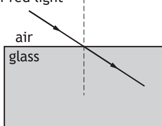
B ray of red light
